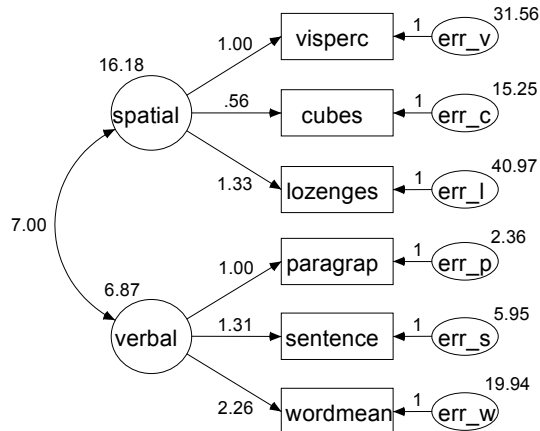
Example 12: Model B Factor analysis: Boys' sample Holzinger and Swineford (1939) Unstandardized estimates
